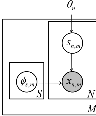
Fig. 5 Graphical model for the standard stel model
