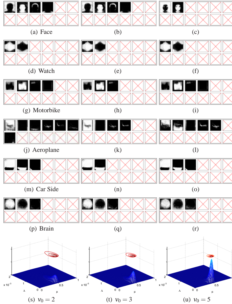
Fig. 13 Inferred stels for different settings of v_0 across columns. The other NIW parameters are set to \{\mu_0 = 0.5, \Lambda_0 = 0.001, \kappa_0 = 0.1\}
